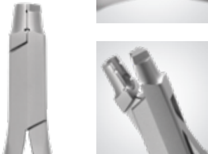
3000/29 Schwarz ø max 0,7 mm / .028" mm 125 Arrow clasp former plier.
