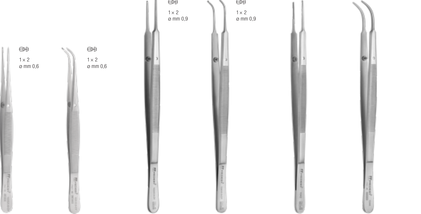
1035/0,6-0Y Semken Straight Retta mm 125 1031/0,6-0Y Semken Curved Curva mm 125 1020/0,9-0Y Gerald Straight Retta mm 175 1040/0,9-0Y Gerald Curved Curva mm 175 1042 Gerald Straight Retta mm 175 1044 Gerald Curved Curva mm 175
